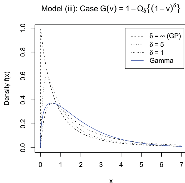
Figure 3. Density function corresponding to Model (6) combined with G(v) = 1 - Q_{\delta}\{(1-v)^{\delta}\} , for \sigma = 1 , \xi = 0.5 and parameters \delta = 1, 5, \infty (dashed-dotted, dotted, dashed black curves, respectively). The limiting case \delta = \infty corresponds to the exact GP density. The solid blue curve represents a gamma density with parameters (1.4, 1.4).
