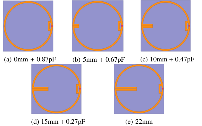
Fig. 4: The antenna for the five capacitor configurations.
