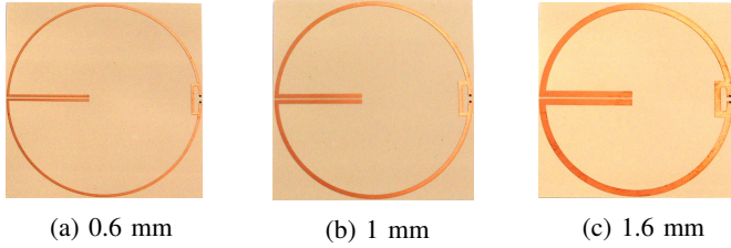
Fig. 2: The three realized antennas with different strip widths.
