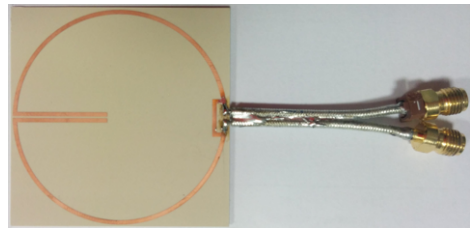
Fig. 1: Picture of the realized electrically small antenna fed by joint coaxial cables used for experimental characterization.
