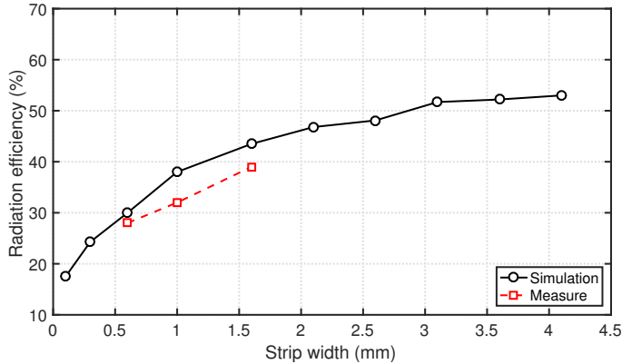
Fig. 3: The antenna radiation efficiency as a function of the strip width. Simulation and measurement.
