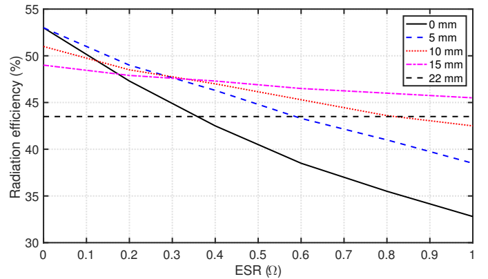
Fig. 5: Radiation efficiency as a function of the capacitor ESR for the five different configurations.
