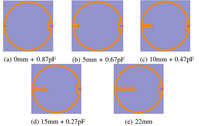
Fig. 4: The antenna for the five capacitor configurations.
