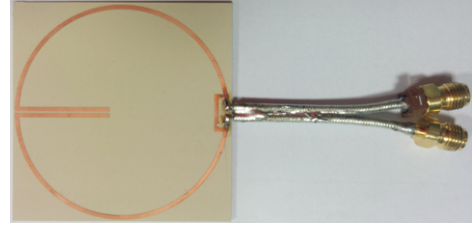
Fig. 1: Picture of the realized electrically small antenna fed by joint coaxial cables used for experimental characterization.
