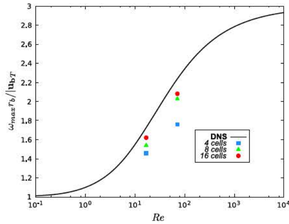
Fig. 27. Single bubble rise. Normalized vorticity \omega_{max} r_b / |\mathbf{u}_b T| for Re = 17 and Re = 71 .
