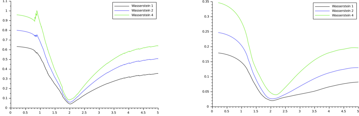
FIGURE 3. \vartheta \mapsto \mathcal{F}_{d_{CF,2}}(\vartheta) for H = 0.3 (left) and H = 0.7 (right).
