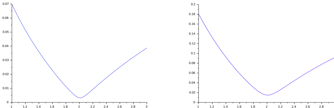
FIGURE 1. \vartheta \mapsto \mathcal{F}_{d_{CF,2}}(\vartheta) for H = 0.3 (left) and H = 0.7 (right).
