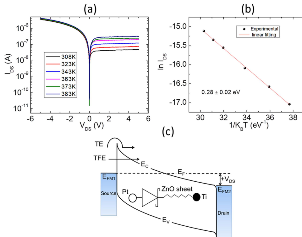
Figure 4. (a) I - V characteristics of Pt-ZnO contact as a function of temperature from 308 to 383 K. (b) Arrhenius plot. The activation barrier energy is extracted from the plot by measuring the slope of the curve which comes to be 0.28 \pm 0.02 eV. (c) Simplified energy band diagram for Pt-ZnO-Ti system under thermal equilibrium at positive V_{DS} . Also schematically showing the two dominant charge carrier injection mechanism (TE and TFE) at reverse biased Schottky contact. E_{FM1} and E_{FM2} are the Fermi level for metals Pt and Ti, respectively.
