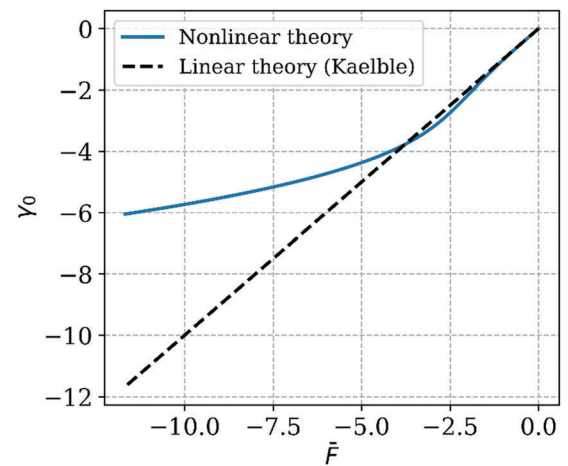
Fig. 3 Normalized peel force \bar{F} versus maximum shear strain \gamma_0 at the peel front. Nonlinear theory and linear theory (Kaelble) predictions, for various \bar{F} , are plotted as solid and dashed lines respectively.
