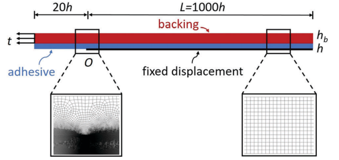
Fig. 5 Schematic of a finite element model and mesh strategy. The red and blue filled rectangles represent the backing layer and adhesive layer respectively, and the rigid substrate is modeled by the fixed displacement boundary condition.
