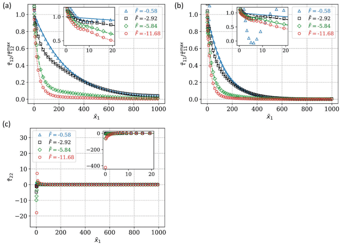
Fig. 7 True stress along the adhesive/substrate interface with different applied loads. Analytic solutions and FEM results are plotted as lines and symbols for different applied forces, i.e. , \bar{F} = -0.58, -2.92, -5.84 and -11.68 respectively. The true stresses near the origin are plotted in the insets: (a) \bar{\tau}_{12}/\bar{\tau}_{12}^{\max} , (b) \bar{\tau}_{11}/\bar{\tau}_{11}^{\max} , and (c) \bar{\tau}_{22} .
