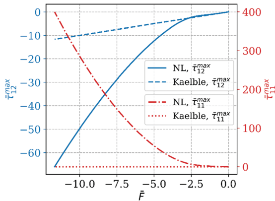
Fig. 4 Normalized peel force \bar{F} versus maximum normalized shear \bar{\tau}_{12}^{\max} (solid blue line) and lateral normal stress \bar{\tau}_{11}^{\max} (dashed-dotted red line). The linear theory of Kaelble is plotted as dashed and dotted lines. Note that the linear theory assumes \tau_{11} = 0 .
