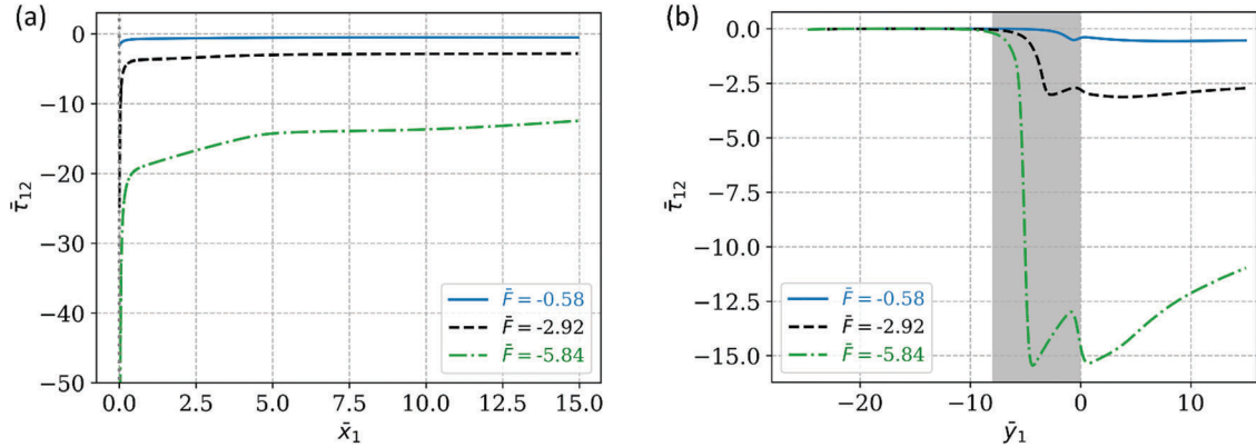
Fig. 9 \bar{\tau}_{12} along the adhesive/substrate and adhesive/backing with different applied forces. FEM results are plotted as solid, dashed and dashed-dotted lines for \bar{F} = -0.58, -2.92 and -5.84 respectively. (a) \bar{\tau}_{12} along the adhesive/substrate interface. (b) \bar{\tau}_{12} along the adhesive/backing interface.
