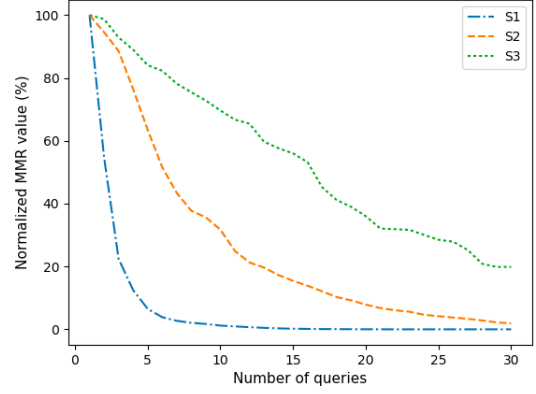
Figure 3: Elicitation with S1, S2, S3 (10 agents, 50 items)
