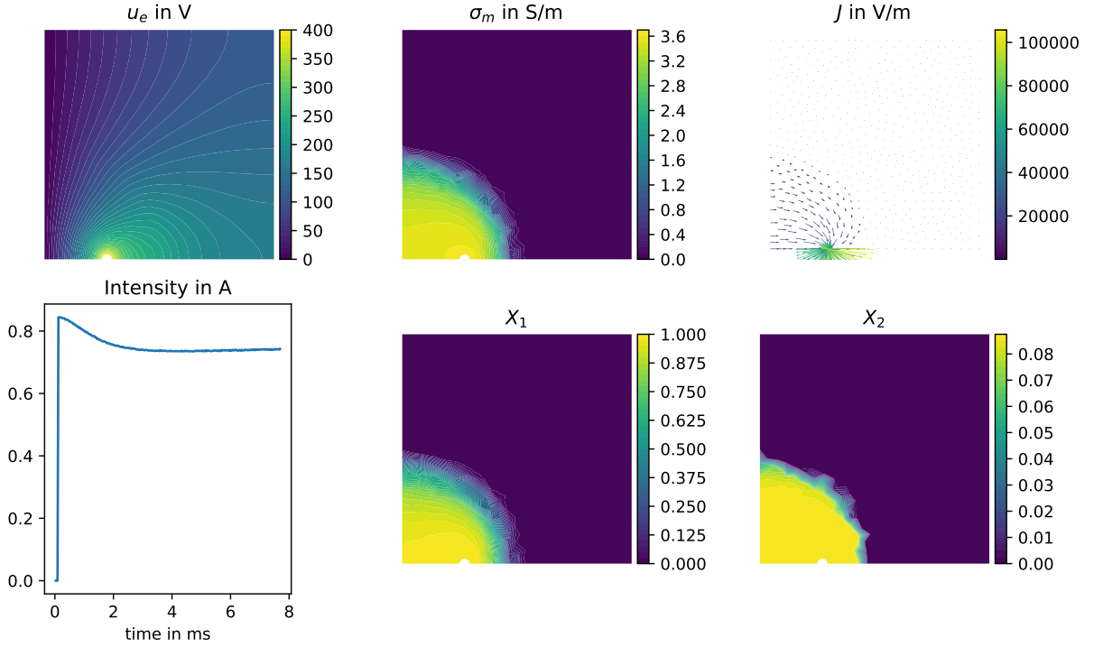
FIGURE 8. Solution to the biphasic model at around 8ms, using the parameters of [20, Table 1], with a 800V voltage step. It is easy to see that \sigma_m is mainly driven by the value of X_1 , i.e. the poration process. At the lower left is the evolution of the current intensity flowing through the electrodes, the spike qualitatively matches experiments, see [20].
