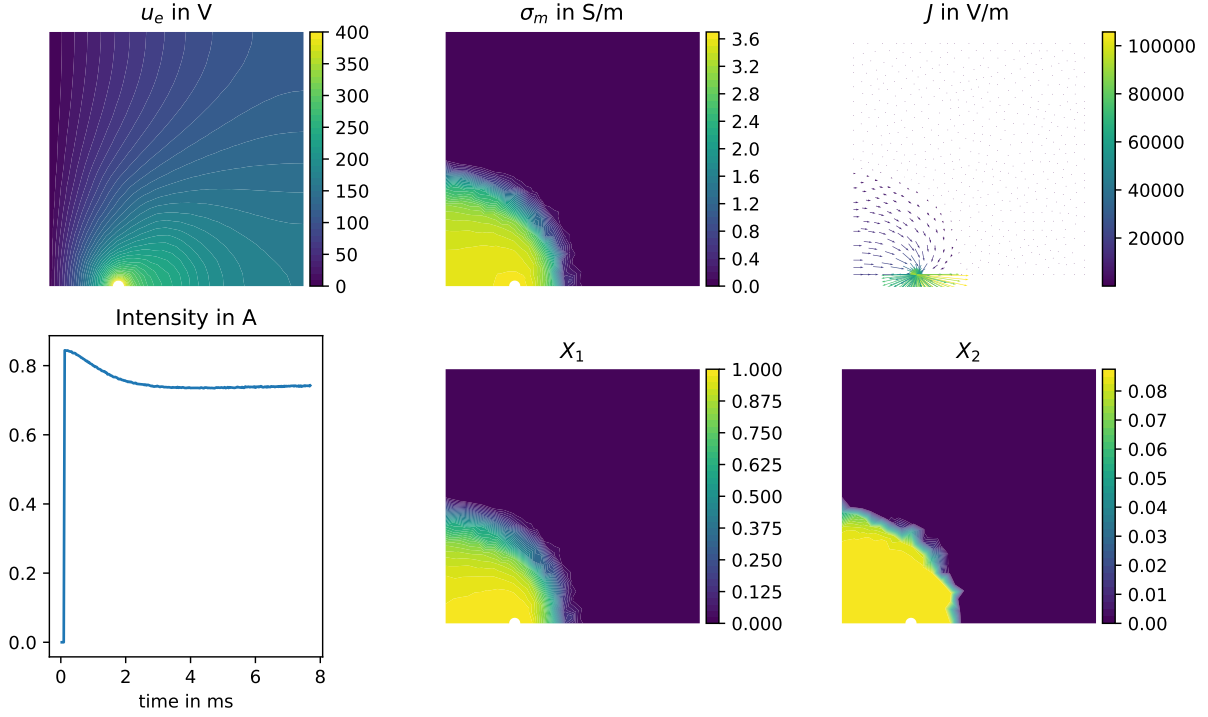
FIGURE 7. Solution to the biphase model at around 8ms, using the parameters of [18, Table 1], with a 800V voltage step. It is easy to see that \sigma_m is mainly driven by the value of X_1 , i.e. the poration process. At the lower left is the evolution of the current intensity flowing through the electrodes, the spike qualitatively matches experiments, see [18].
