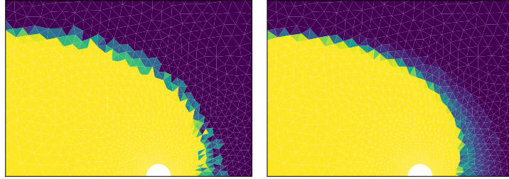
FIGURE 4. Comparison of \sigma(\|\nabla u\|) for typical solutions of 1 given by the evolution-based iterative method (left) and the Newton's approach (right) for the standard model.
