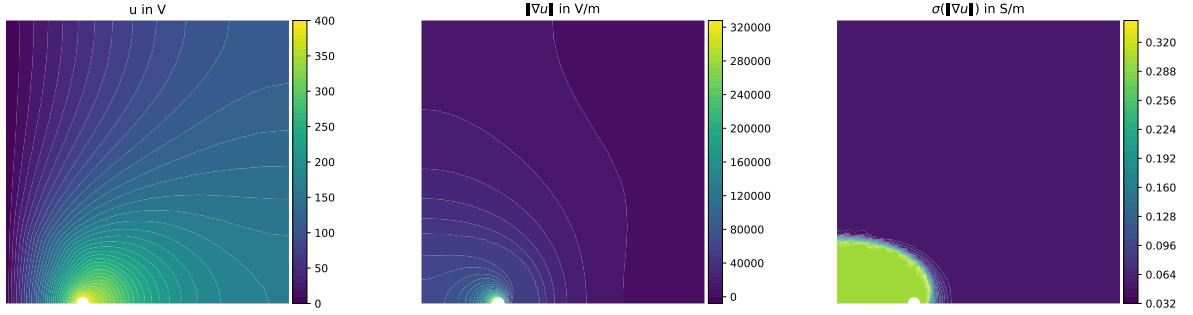
FIGURE 5. Solution of the static standard model, using parameters E_{th} = 5.75 \times 10^4 V/m , k_{ep} = 10^{-3} V^{-1} , \sigma_0 = 0.065 S/m and \sigma_1 = 0.1483 S/m .
