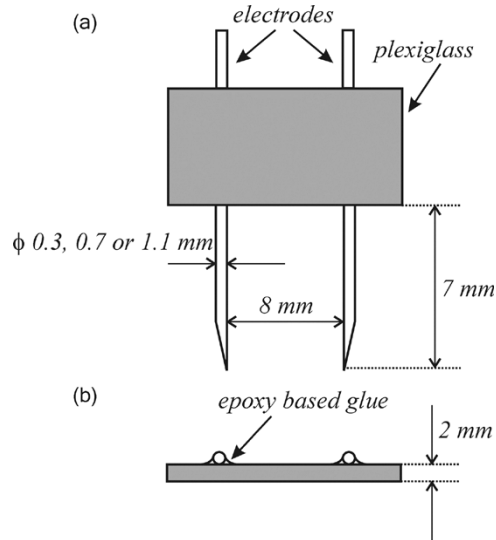
FIGURE 2. Experimental set-up for electroporation measurements as performed by Sel et al. 3 electrodes diameter are considered. The piece of rabbit liver is located below the plexiglass on a thickness of 7 mm [17].
