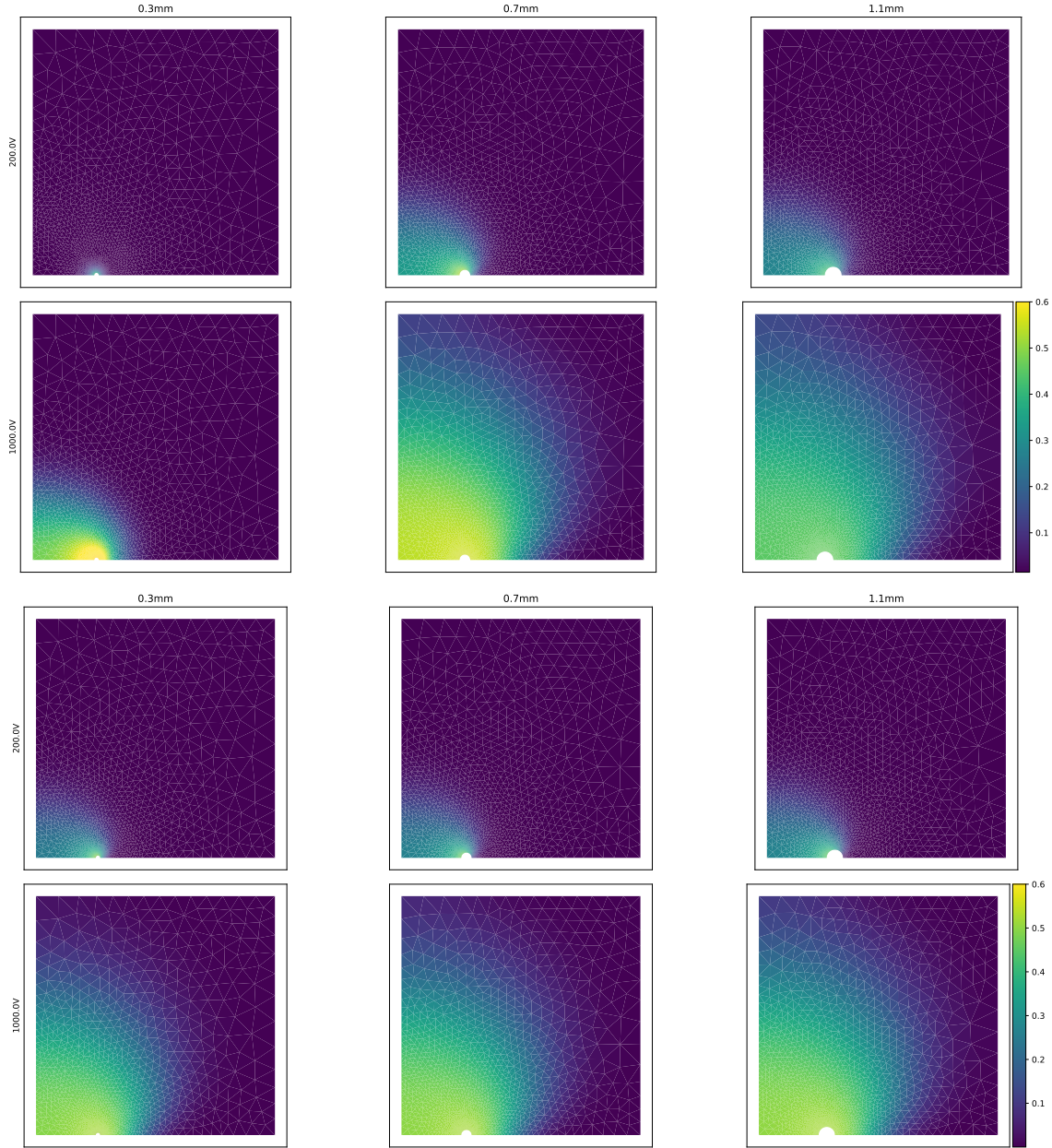
FIGURE 10. \sigma(\|\nabla u\|) in S/m for applied voltages 200V and 1000V and the three geometries, for the parameters estimated separately on each geometry (top 2 lines) and for the parameters estimated on all geometries simultaneously (bottom 2 lines).
