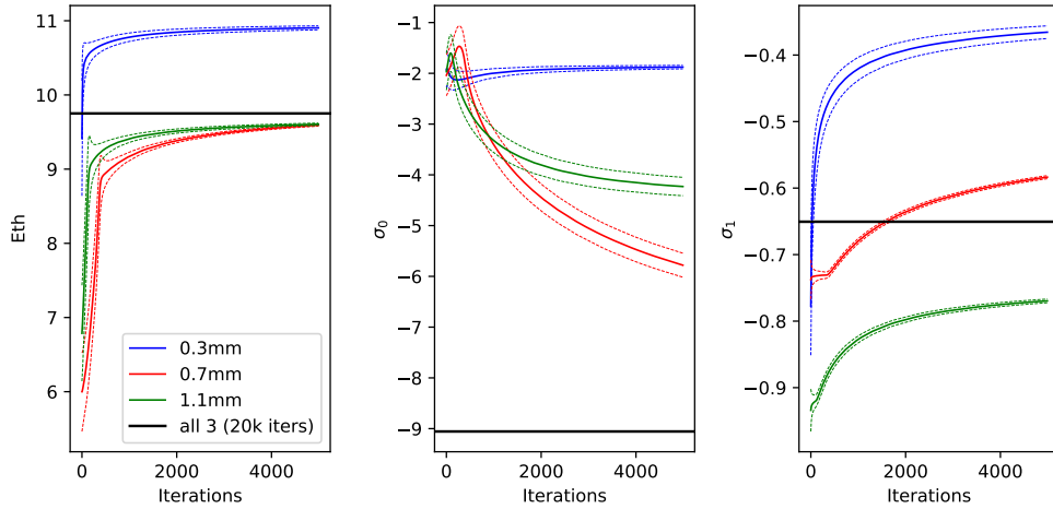
FIGURE 9. Estimation of E_{th} , \sigma_0 and \sigma_1 , after log-transformation. All voltages are considered, but electrode diameters are considered separately. The thin lines denote the standard deviation of the uncertainty on the estimation.
