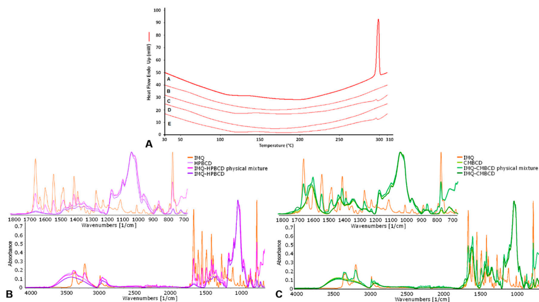
Figure 2. (A) Differential scanning calorimetry (DSC) thermograms of imiquimod (IMQ) and IMQ inclusion complexes: (A) IMQ, (B) IMQ–HP \beta CD, (C) IMQ–HP \beta CD physical mixture, (D) IMQ–CM \beta CD, (E) IMQ–CM \beta CD physical mixture; (B) Attenuated total reflection–Fourier transformed infrared (ATR–FTIR) spectra of IMQ and HP \beta CD complex; (C) Attenuated total reflection–Fourier transformed infrared (ATR–FTIR) spectra of IMQ and CM \beta CD complex.
