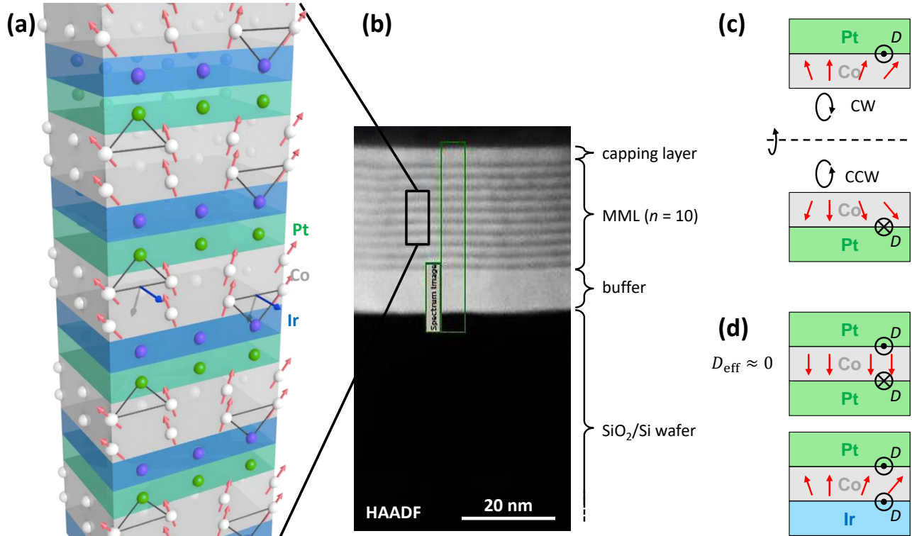
Figure 1. Structure of the studied samples. (a) Artistic representation of the magnetic multilayers made of repetitions of Pt|Co|Ir. (b) Actual transmission electron microscopy cross-section displaying continuous Co layers, nominally 0.8-nm thick. (c-d) Illustration of the need to have different top and bottom interface to obtain large effective DMI: (c) by symmetry, rotating the sample around the dashed line, one easily verifies that the DM vector changes sign for the top interface and hence compensates the DM vector of the bottom interface. (d) Choosing a material with opposite D , on the contrary, allows one to enhance the DMI.
