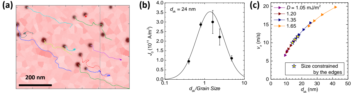
Figure 7. Current-induced skyrmion motion in a system with non-uniform crystalline grain distribution. (a) Image of a simulation landscape (grains of different pink levels are grains with different D , 10% variation considered here). The trajectories (colored lines) are calculated using micromagnetic calculations, skyrmions are drawn at their initial position. (b) “Depinning” current as a function of the ratio between the skyrmion diameter and the grain sizes. (c) Skyrmion velocity as a function of skyrmion diameter at an edge or in a track.
