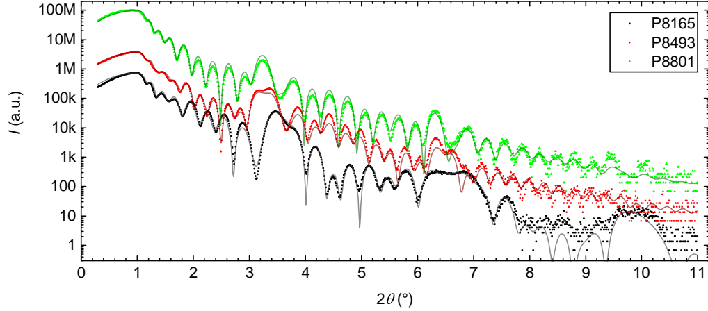
Figure 2. Low angle X-ray reflectivity (using a laboratory \text{Cu } K_{\alpha} source) of a series of five repetitions samples with nominal composition: P8165 \|\text{Pt}10\|(\text{Ir}1|\text{Co}0.8|\text{Pt}1)\times 5|\text{Pt}3 , P8493 \|\text{Ta}5|\text{Pt}10\|(\text{Co}0.8|\text{Ir}1|\text{Pt}1)\times 5|\text{Pt}3 , and P8801 \|\text{Pt}11\|(\text{Co}0.8|\text{Ir}1|\text{Pt}1)\times 5|\text{Pt}3 (numbers after the elements are thicknesses in nm and \|\text{Pt}10\| designates the \text{SiO}_2 substrate, a.u. stands for arbitrary units, \theta is the X-ray incidence angle). Experimental data are fitted using X'Pert Reflectivity PANalytical software, which confirms the nominal multilayer thicknesses.
