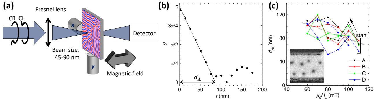
Figure 3. Scanning X-ray transmission microscopy using circularly polarized light. (a) Schematic view of the measurement setup: X-ray at the \text{Co } L_3 edge energy is focused on the sample, which is scanned in the beam, and the transmitted photon intensity is measured. An external magnetic field can be applied perpendicular to the sample. (b) Profile of a skyrmion as measured by STXM. The angle \theta with the normal to the film as a function of the skyrmion radius r is deduced from m_z , which is obtained by deconvoluting the difference in absorption for CL and CR light. (c) Measurement of four skyrmion diameters d_{\text{sk}} as a function of the out of plane magnetic field. Inset: corresponding STXM dichroic image, 1.4 \times 1.4 \mu\text{m}^2 .
