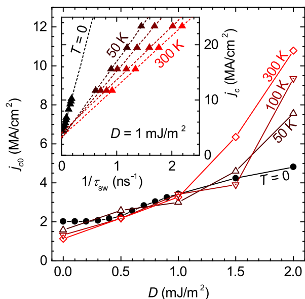
FIG. 3. Effects of DMI on the thermal stability and current induced switching of MRAMs. j_{c0} versus D for T = 0, 50, 100 , and 300 K. The inset plot is the current versus the reciprocal mean switching time ( \tau_{sw} ) for D = 1 mJ/m 2 , for temperatures of 50, 100, 200 , and 300 K, extracted from multiple (60 to 80) stochastic simulations; the data for T = 0 are also shown.
