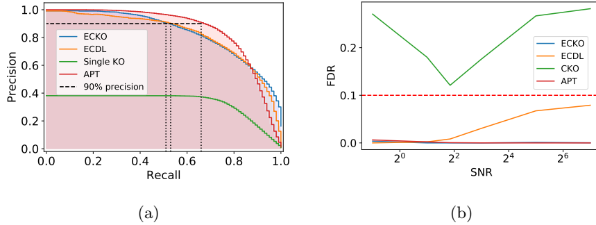
Fig. 3: (a) Average Precision-recall curve (for SNR \approx 3.6 ) and (b) SNR-FDR curve of 30 synthetic simulations. Nominal FDR control level is 10%. ECKO shows substantially better results than CKO and is close to ECDL. APT obtains a slightly better Precision-recall curve. ECKO, ECDL and APT successfully control FDR under nominal level 0.1 where as CKO fails to.
