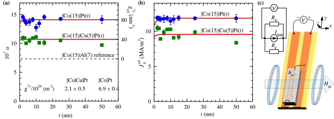
Figure 5: Results extracted from the FMR measurements on strip-line (for frequency dependence) and in cavity (for proper estimation of h_{\text{rf}} and large Q ). (a) Platinum thickness dependence of the damping and the corresponding spin mixing conductance. The damping is essentially constant down to 2 nm of Pt. (b) Estimated effective spin current as calculated from Eq.4. The behavior of the effective spin current follows the one of the damping; no clear variation with thickness down to 2 nm is detectable. The fits (red lines) of both (a) and (b) are calculated using Eq.10 which takes in account the spin memory loss. (c) Equivalent circuit used to analyze the data in the spin-pumping-ISHE configuration, and schematics of the used experimental setup. For practical reasons, the sample is glued on a PCB (yellow) with two Cu conducting lines (orange) that are connected by wire bonding (grey) at the edges of the sample. The sample and the PCB are inserted in a half-cylinder resonant cavity (not shown) that generates the rf magnetic field h_{\text{rf}} . The whole system is placed inside large coils (blue) that generate the quasi-static magnetic field H_{\text{dc}} . H_{\text{dc}} is swept at less than 500 (A/m)/s, and both the dc voltage V and the absorption of the rf field are monitored simultaneously.
