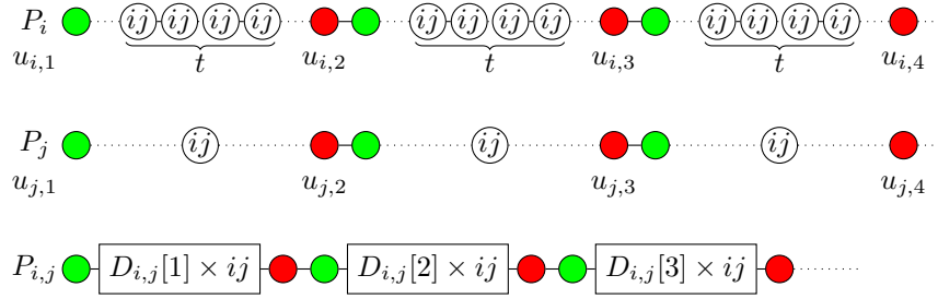
Figure 7: The oriented paths P_i , P_j , and P_{i,j} . Again, color c_b is represented in green (light gray) and color c_e in red (dark gray). Note that the P_i 's do depend only on the number t of vertices per color class, while P_{i,j} actually encodes the adjacency between H_i and H_j in some flattened form.
