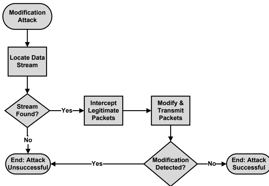
Figure 3. Data modification attack.
