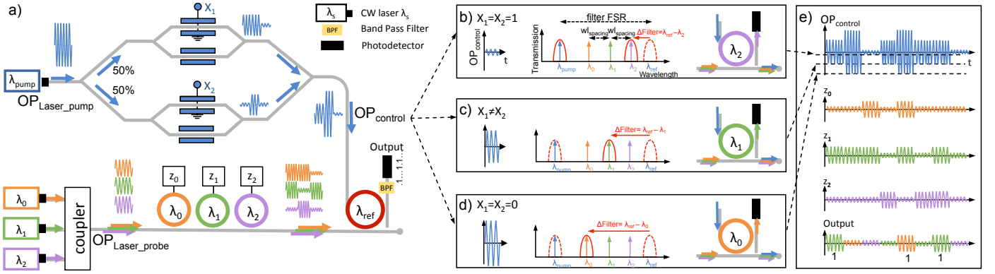
Fig. 3: Optical SC unit of a 2 nd order polynomial function. a) The optical circuit. The transmissions of the signals at \lambda_2, \lambda_1 , and \lambda_0 to the drop port of the filter are shown in b), c), and d), respectively. e) Transmission example of the probe and control signals, and power received by the photodetector.
