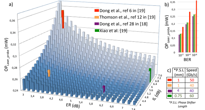
Fig. 6: Minimum probe laser power according to a) IL_{\text{dB}} and ER_{\text{dB}} for 10^{-6} BER b) targeted BER, and c) MZI speed and phase shifter length.
