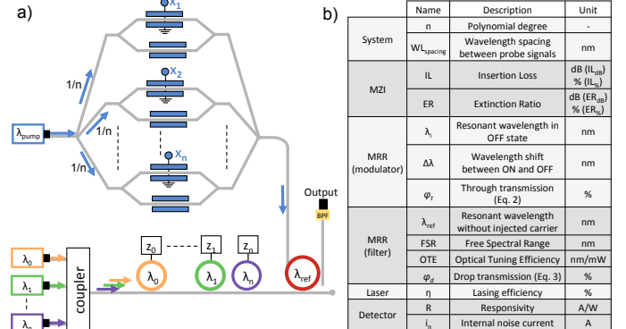
Fig. 4: a) Generic architecture for optical stochastic computing circuit, and b) System-level and device-level parameters.
