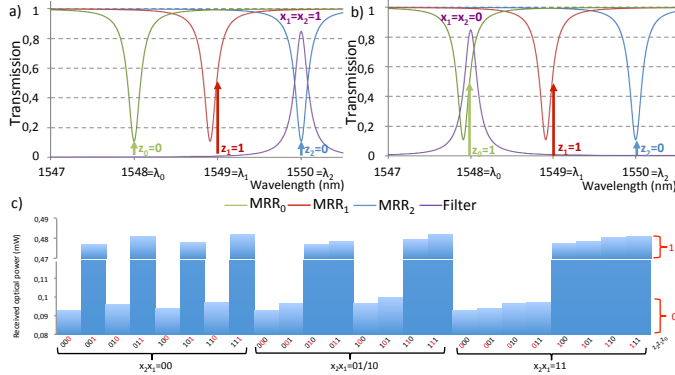
Fig. 5: Transmission of MRRs and filter. a) probe signal at \lambda_2 is transmitted as 0, b) probe signal at \lambda_0 is transmitted as 1, and c) The optical power received by the photodetector for all input combinations.
