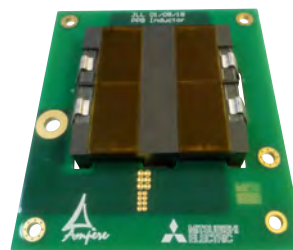
Figure 2: Example of planar inductor
