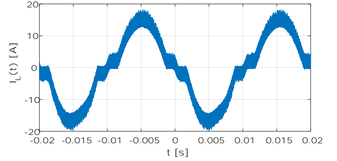
(b) Inductor current 10.3 A_{RMS}
