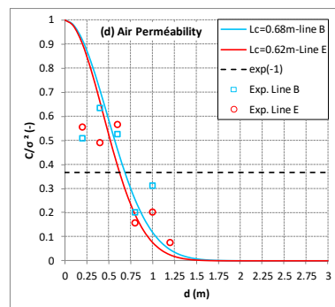
Fig. 7. Correlation length identification of the air permeability
