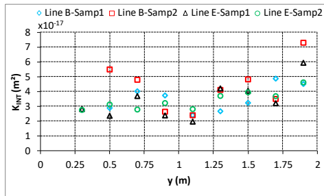
Fig. 4. Intrinsic permeability following the vertical lines B and E
