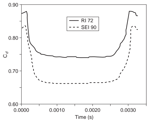
Figure 6 Computed discharge coefficient during the injection process.
