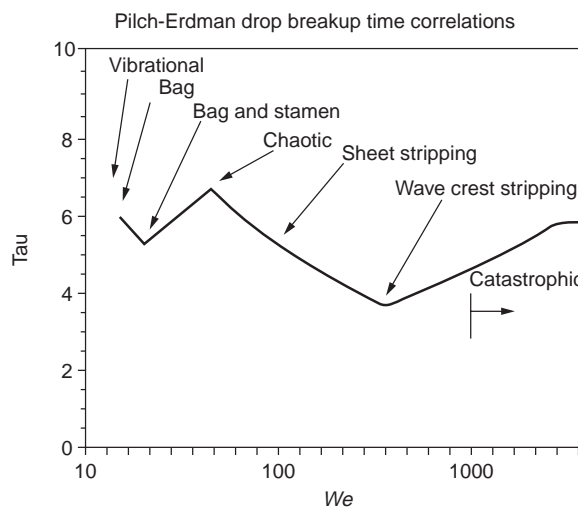
Figure 5 Drop secondary breakup timescales.
