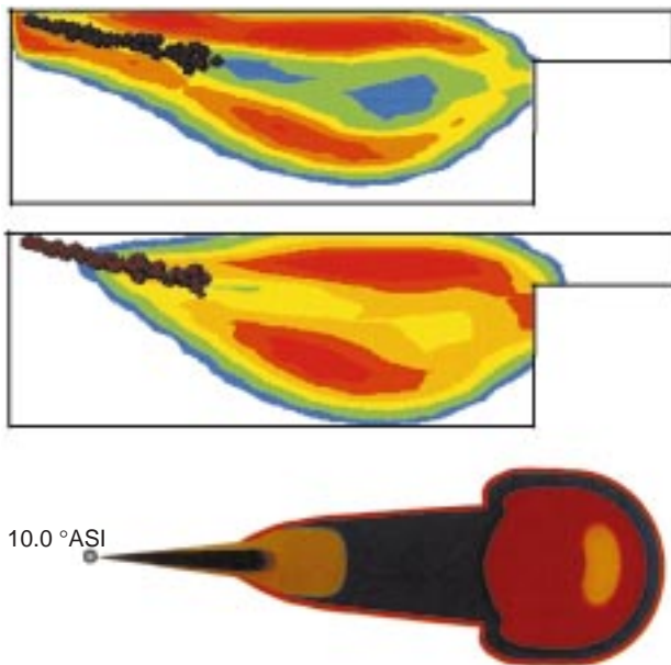
Figure 9 Temperature distribution for the baseline case (top), with nozzle flow model (middle), experimental soot image (bottom – Dec, 1997) at 10 ASI.
