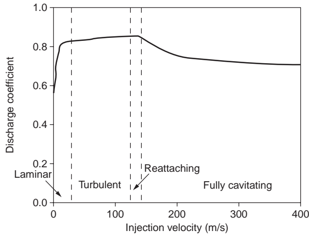
Figure 1 Discharge coefficient variation in different flow regimes.
