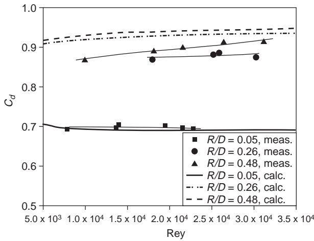
Figure 2 Comparisons of experimental and model results for the influence of R/D on C_d .
