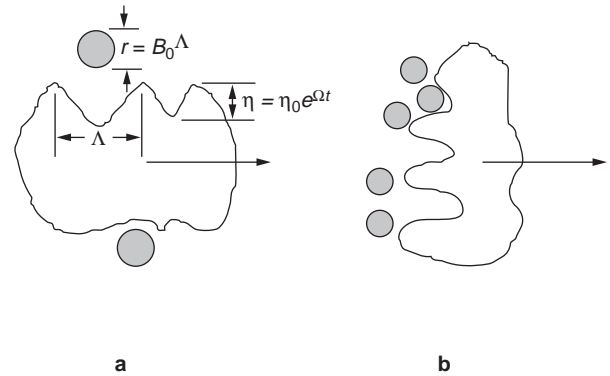
Figure 3 Schematic diagram of drop breakup mechanisms a: KH-type; b: RT-type.
