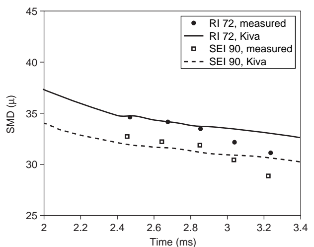
Figure 7 Comparison of measured and computed SMD.
