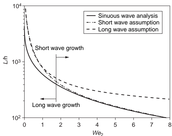
Figure 4 Dimensionless breakup length as a function of sheet Weber number, We_2 .
