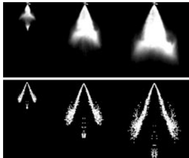
Figure 10 Comparisons of photographs (top) and computer model predictions (bottom) for 0.7, 1.7 and 2.7 ms after the start of injection (from left to right). The numerical results present a two-dimensional slice through the spray to show the spray structure.
