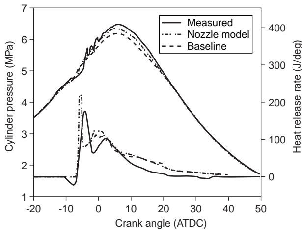
Figure 8 Effects of nozzle flow details on engine combustion simulations.
