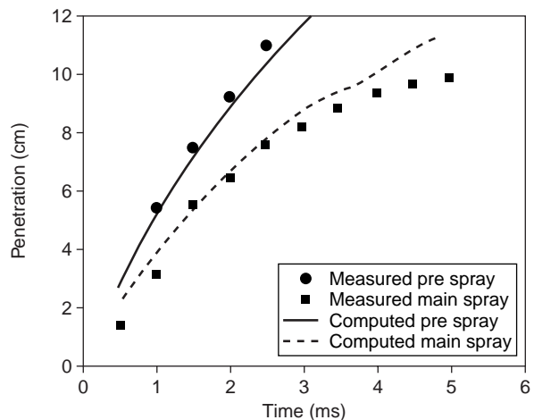
Figure 11 Measured and predicted spray penetration for the main spray and pre-spray as functions of time.
