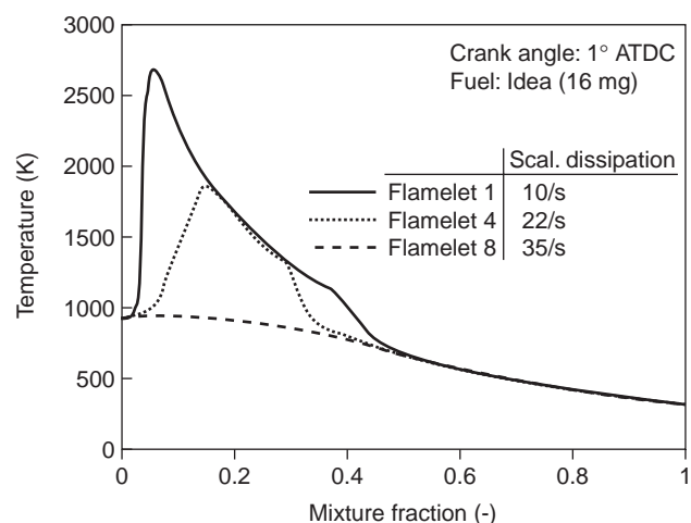
Figure 12 Temperature in different flamelets at 1° CA ATDC.
