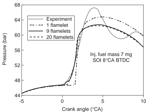
Figure 6 The influence of the number of flamelets on pressure.
