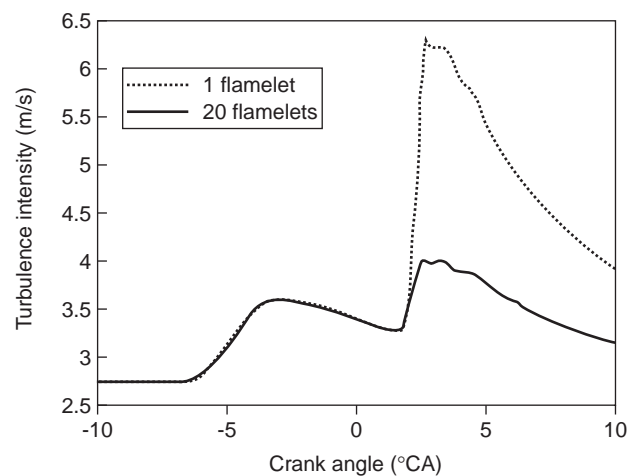
Figure 7 The influence of the number of flamelets on the cylinder averaged turbulence intensity.
