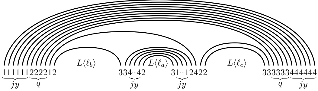
Figure 2: A 3-clause gadget S\langle C_j \rangle : l_a \vee l_b \vee l_c with a < b < c .
