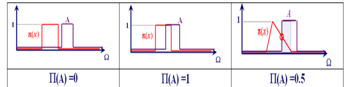
Fig.1 Possibility calculation of an imprecise event A.
