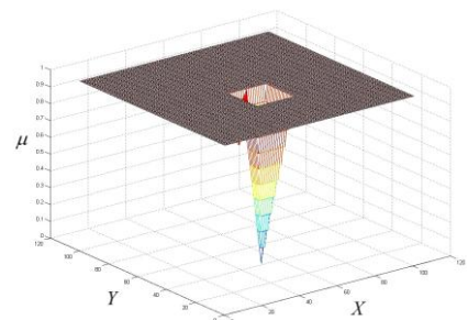
Fig.11 Necessity degree estimation.
