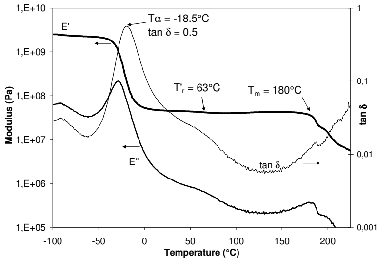
Figure 2. DMTA curves obtained on a mature 2-mm thick plate. (Testing conditions: 0.1% strain, heating rate: 3°C/min, frequency: 1Hz.). T_r is defined as the inflection point of the loss of modulus occurring between 50 and 100°C.
