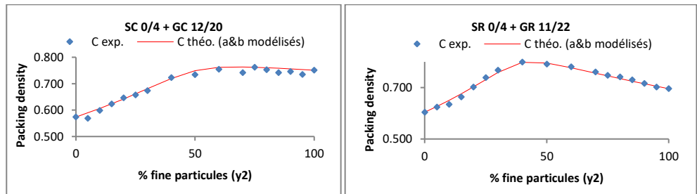
Fig. 7 Measured and modeled packing density of crushed (a) and rolled (b) binary mixtures - Calibrated interaction coefficients on our mixtures.
