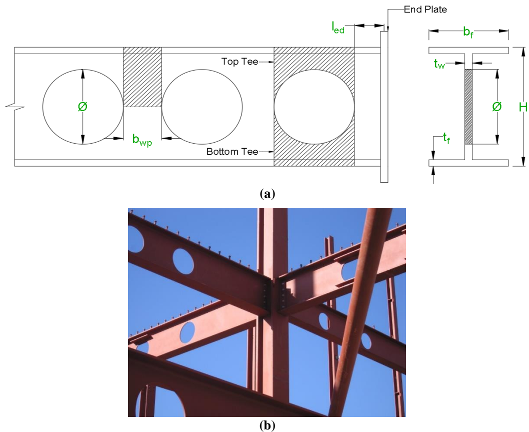
Fig. 1. Steel Cellular Members: (a) input (parametric) variables, and (b) application in an office building floor system in Lisbon, Portugal.
