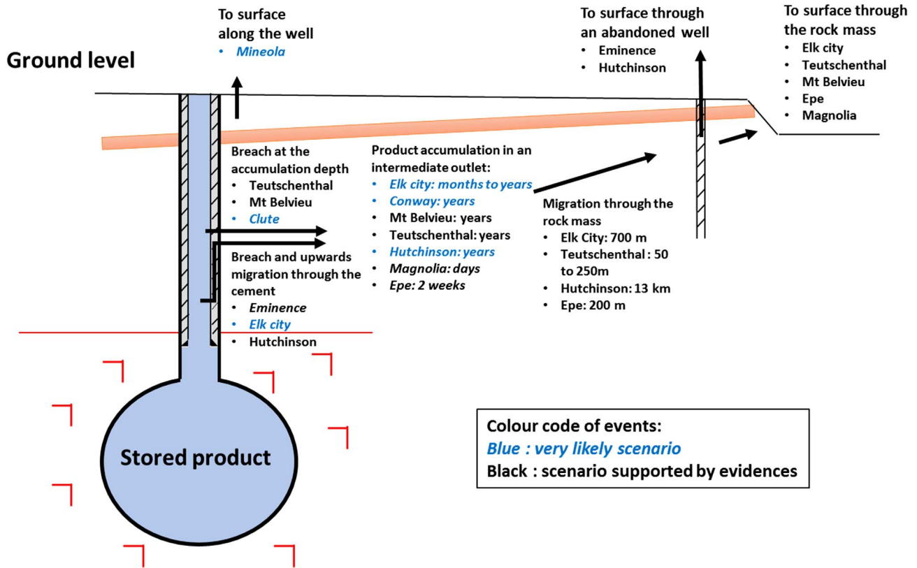
Fig. 13. Schematic of leakage development cases with an intermediate outlet accumulation.
