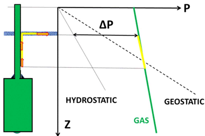
Fig. 16. A gas leaks from a breach in the casing. Gas migrates through the cement and reaches a shallower aquifer layer, at which point its pressure is much higher than in situ groundwater pressure and even, in many cases, higher than geostatic pressure.
