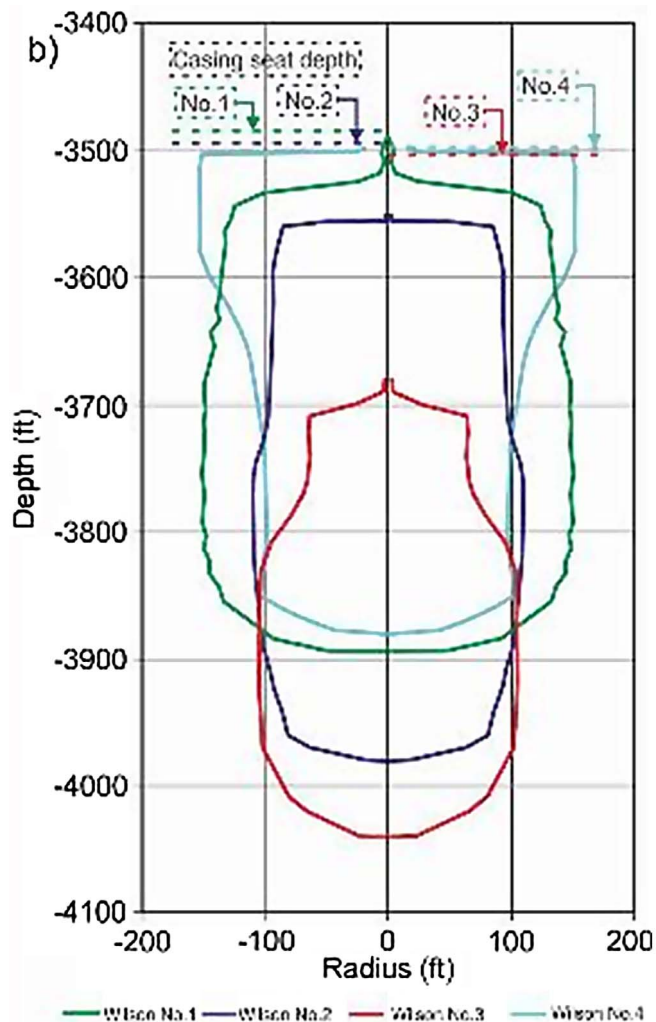
Fig. 9. General cross-sections of caverns, based on sonar data. From Osnes et al. (2007)
