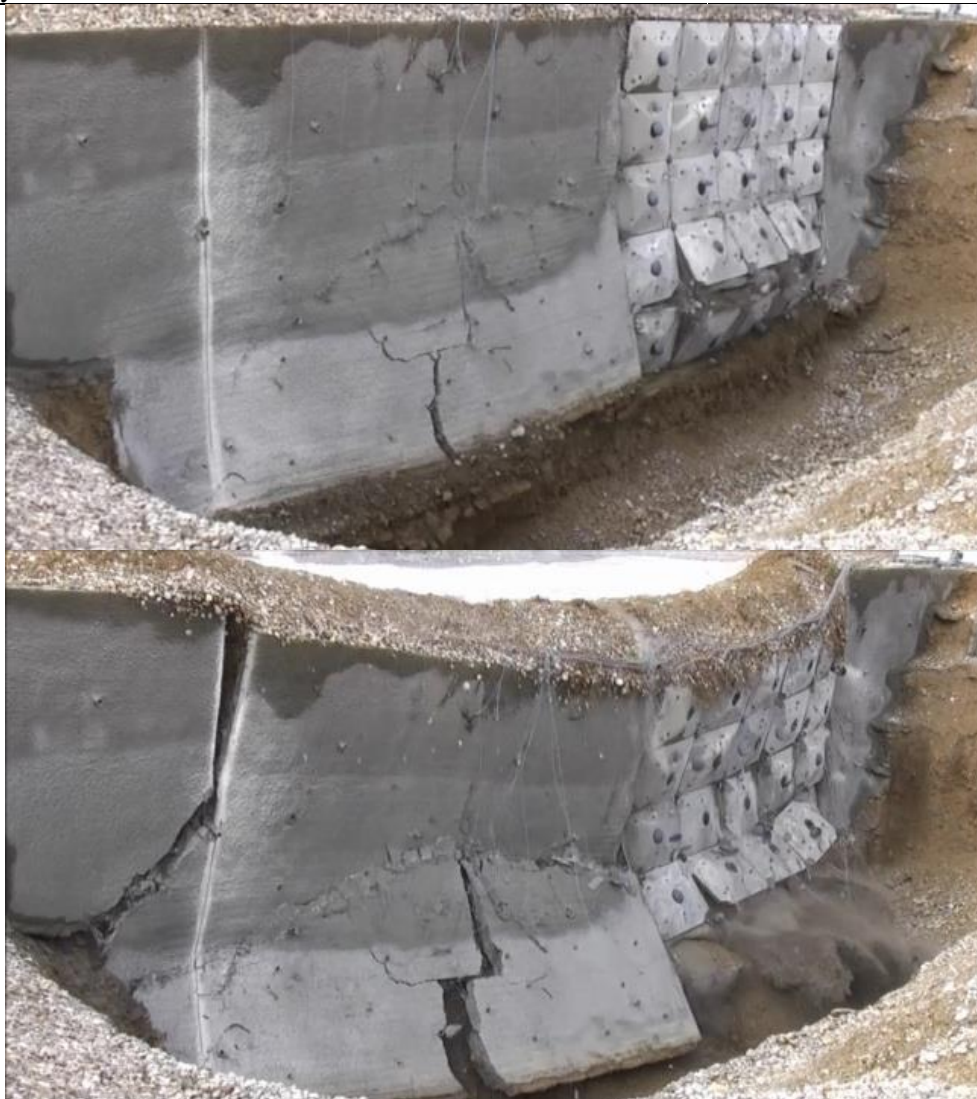
Figure 11. Collapse mode of two nail walls under explosion
