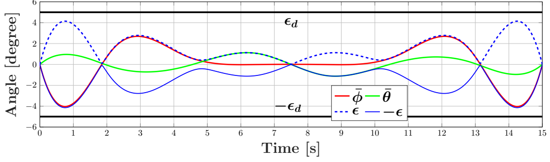
Figure 5. Roll, pitch angles references \bar{\phi}, \bar{\theta} , and the angle boundary \epsilon as in (12) compared with the desired angle limit \epsilon_d .
