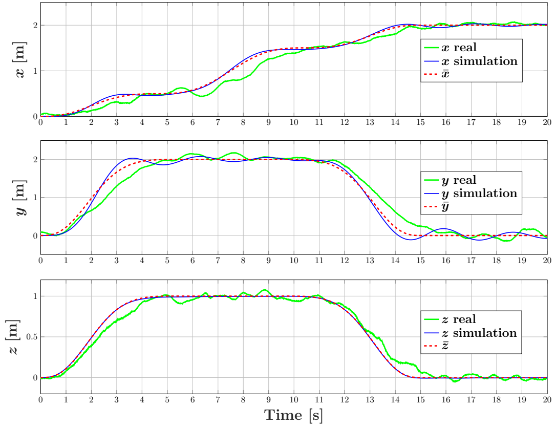
Figure 7. Tracking results of the three axes.
