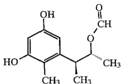
Figure 6. Ring opening of citrinin (citrinin H2) induced by increase of pH [56].
