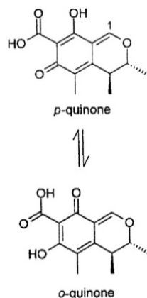
Figure 2. Chemical structure of citrinin, existing in both forms.
