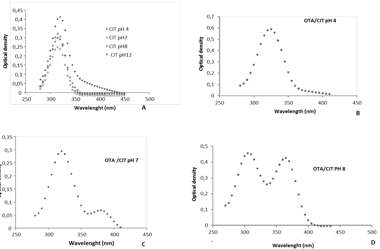
Figure 4. UV-Spectra of citrinin and ochratoxin A in mixture: Curve A represents the spectrum of CIT at four pH (4, 7, 8 and 12). Curve B represents the spectrum of CIT in mixture with OTA at pH 4. Curve C represents the spectrum of CIT in mixture with OTA at pH 7. Curve D represents the spectrum of CIT in mixture with OTA at pH 8.
