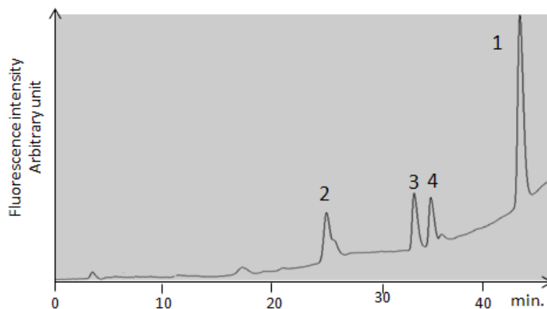
Figure 7. HPLC separation of OTA metabolites from the mixture of OTA and citrinin in aqueous solution.
