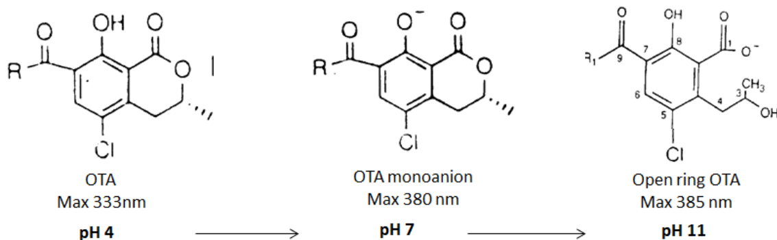
Figure 5. Ring opening of OTA (OP-OA) under alkaline conditions adapted from [50–52].
