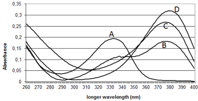
Figure 4. UV-Spectra of citrinin and ochratoxin A in mixture: Curve A represents the spectrum of CIT at four pH (4, 7, 8 and 12). Curve B represents the spectrum of CIT in mixture with OTA at pH 4. Curve C represents the spectrum of CIT in mixture with OTA at pH 7. Curve D represents the spectrum of CIT in mixture with OTA at pH 8.
