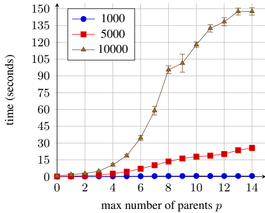
Figure 5. Learning time when the number of variables is fixed ( n = 15 ). We increase the number of objects in the datasets. Results correspond to one learning execution averaged on 2 \times 5 runs and error bars correspond to the standard deviation of the observed values.
