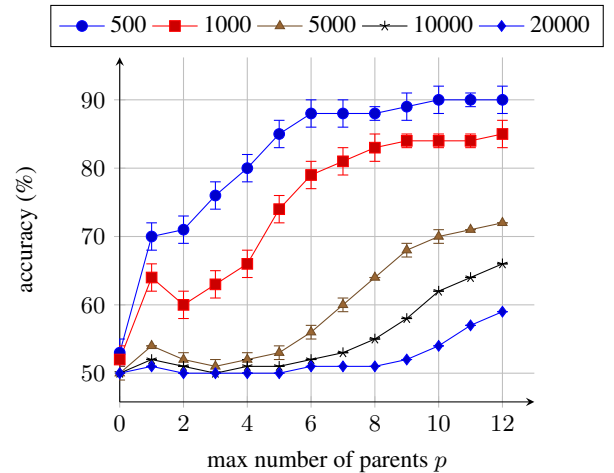
Figure 4. Learning accuracy when the number of variables is fixed ( n = 15 ). We increase the number of objects in the random datasets. Results are averaged on 2 \times 5 runs and error bars correspond to the standard deviation of the observed values.
