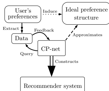
Figure 1. General scheme of a learning procedure for CP-nets.
