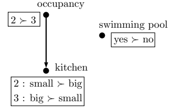
Figure 2. Complete CP-net with three variables.
