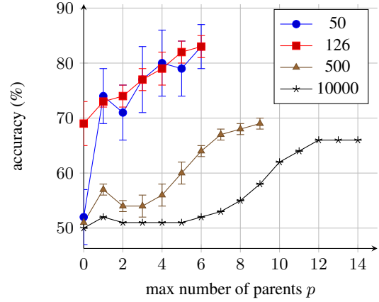
Figure 3. Learning accuracy according to the number of parent p per variable. Datasets are randomly generated except for the real 126 hotels file. Results are averaged on 5 \times 10 runs and error bars correspond to the standard deviation of the observed values.
