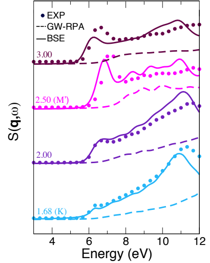
FIG. 3. Dynamic structure factor for \mathbf{q} along \Gamma\text{K} direction calculated in the GW-RPA and from the solution of the BSE compared to the NRIXS data from Ref. 19 . The \mathbf{q} = 2.5 \text{ \AA}^{-1} is the \text{M}' point (see text).
