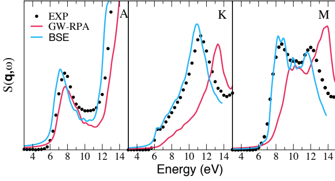
FIG. 1. Dynamic structure factor at three Brillouin zone boundaries \mathbf{q} = \text{A} , \text{K} , and \text{M} calculated in the GW-RPA and from the solution of the BSE compared to the NRIXS data from Ref. 19 .
