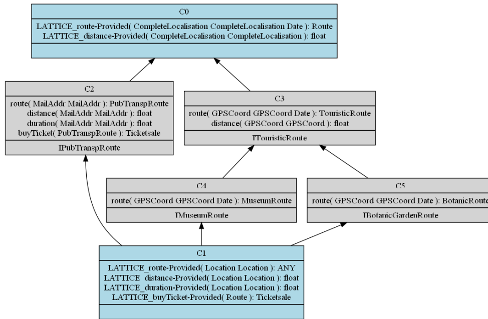
Figure 14 – The \mathcal{L}_{routeInterface} lattice of provided interfaces about routes
