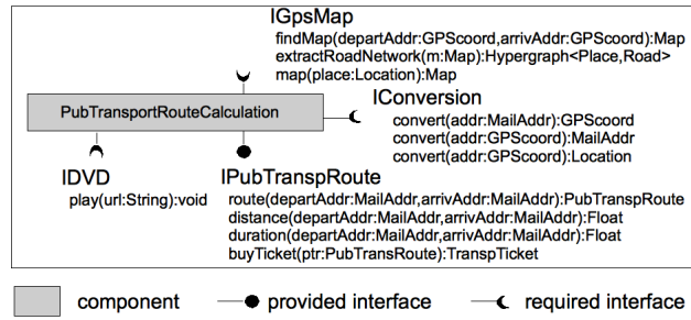
Figure 1 – A component for public transportation route calculation
