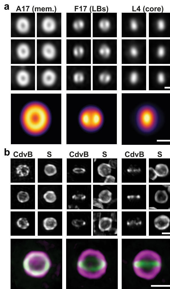
Figure 6. Quantitative SPA-based modelling with NanoJ-VirusMapper. (a) Top: aligned SIM images of individual vaccinia particles labelled for L4 (core), F17 (LBs) and A17 (membrane, mem.). Bottom: VirusMapper models of the three channels. Scale bars: 200 nm. (b) Top: aligned SIM images of individual Sulfolobus acidocaldarius cells labelled for the S-layer (S) and the archaeal ESCRT-III homolog CdvB (CdvB). Bottom: VirusMapper models of three different orientations of the cells; magenta—S-layer, green—CdvB. Scale bars: 1 \mu m.
