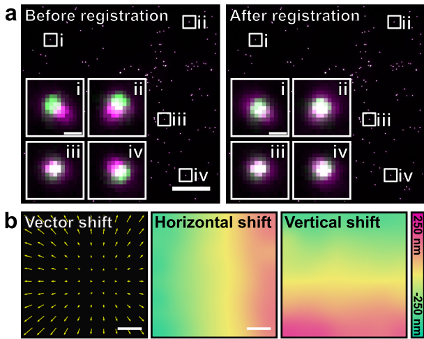
Figure 3. Multi-colour channel registration with NanoJ-Core. (a) Composite image of multi-colour TetraSpeck™ beads imaged in two different channels ('GFP-channel' indicated in green and 'mCherry-channel' in magenta), prior to (left) and after (right) channel registration using NanoJ-Core. Insets—individual beads from indicated locations. Scale bars: 25\ \mu\text{m} , insets: 0.5\ \mu\text{m} . (b) Vectorial representation of the shift between the two channels (left, displacement vector length 50 times larger for representation purposes), horizontal (middle) and vertical (right) shift maps obtained and applied to the data shown in (a). Scale bars: 25\ \mu\text{m} .
