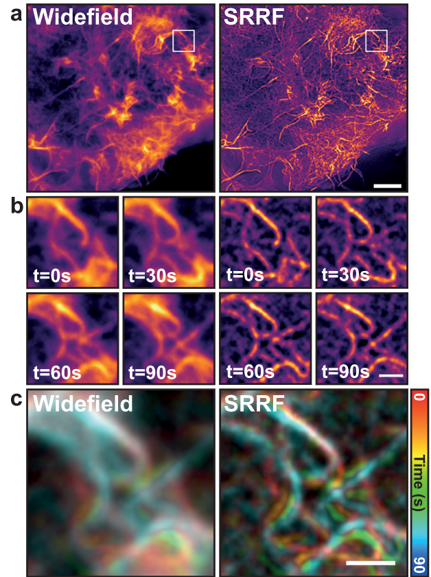
Figure 4. Live-cell SRM with NanoJ-SRRF. (a) Comparison of widefield (left) and SRRF reconstruction (right) obtained from a COS-7 cell expressing UtrCH-GFP to label actin filaments. Scale bar: 5\ \mu\text{m} . (b) Time-course of the inset shown in (a), obtained from a continuous imaging at 30\ \text{ms} exposure ( 33.3\ \text{Hz} ) and displayed every 30\ \text{s} . Scale bar: 1\ \mu\text{m} . (c) Colour-coded time course dataset from (b). Scale bar: 1\ \mu\text{m} .
