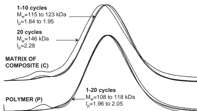
Fig. 6. Exclusion size chromatography elution charts of the dissolved matrices in THF after 1, 5, 10 and 20 cycles.
