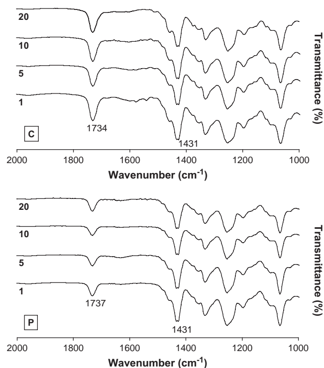
Fig. 7. FTIR spectra of the dissolved samples in THF after filtration of the fibres at 1, 5, 10 and 20 cycles of extrusion and milling. C : composite samples; P : polymer samples. Both samples were analysed after casting of the solution (1% matrix) on a KBr pellet and drying.
