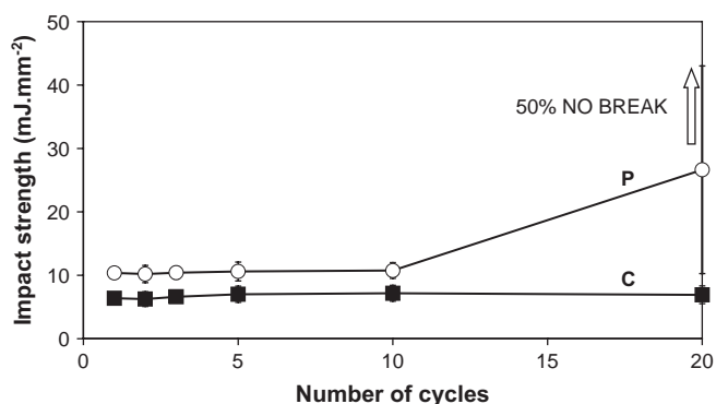
Fig. 3. Impact strength versus the number of cycles. P : polymer; C : composite.
