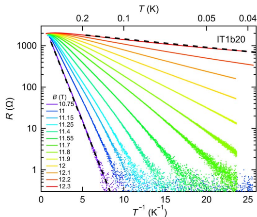
Fig. 2. Fully recovered activated behavior. R versus T^{-1} obtained from IT1b20, an a:InO film, measured with better filtration (see Materials and Methods for details) at different B values. Activated behavior (straight line in an Arrhenius plot) is apparent down to our noise floor or lowest measurement T 's (see, e.g., dashed black lines at B = 10.75 and 12.3 T).
