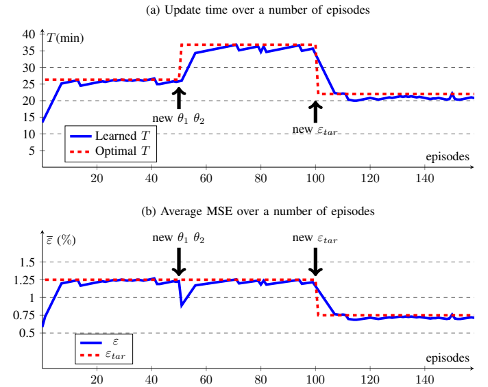
Fig. 6: Updating mechanism searching for the optimal update time, arrows indicate change in the covariance model scaling parameters or \epsilon_{tar} .
