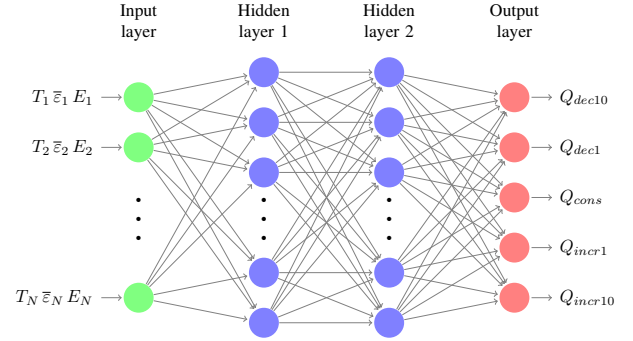
Fig. 4: We employ ANN with two hidden layers, each with 24 neurons. We use MSE loss function and Adam optimization algorithm to train ANN weights. We apply ReLU activation function for the hidden layers and linear activation function for the output layer.
