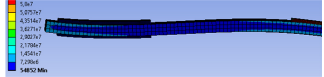
Fig. 6. The bending energy recovery system. The system being symmetrical, only a part has been represented. The equivalent constraints of Von-Mises are represented. The stresses in the piezoelectric are of the order of 50 MPa.
