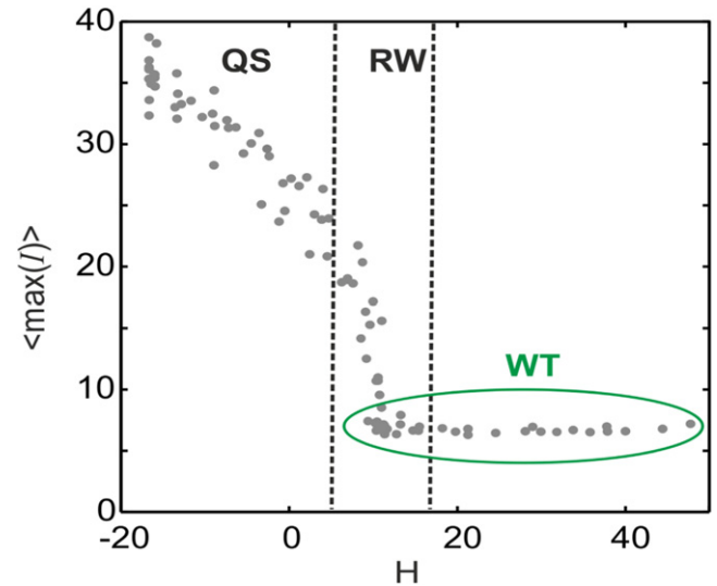
Figure 11. Maximum intensity peak in the simulations of the non-integrable NLSE (with third-order dispersion) by varying the Hamiltonian (‘temperature’), H , keeping fixed the power N = \int I dt , where I = |\Psi|^2 . At small H , regime (QS), a persistent quasi-soliton is generated; at high H , regime (WT), the turbulent system exhibits quasi-Gaussian statistics: short-lived RWs events are essentially generated nearby the transition to quasi-soliton condensation, H = H_c \sim 12 [140].
