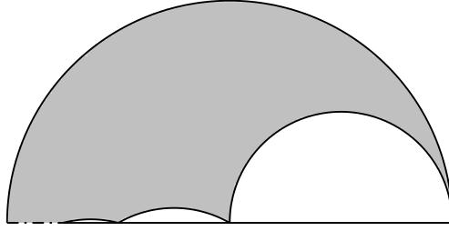
FIGURE 2. The graph of M .
