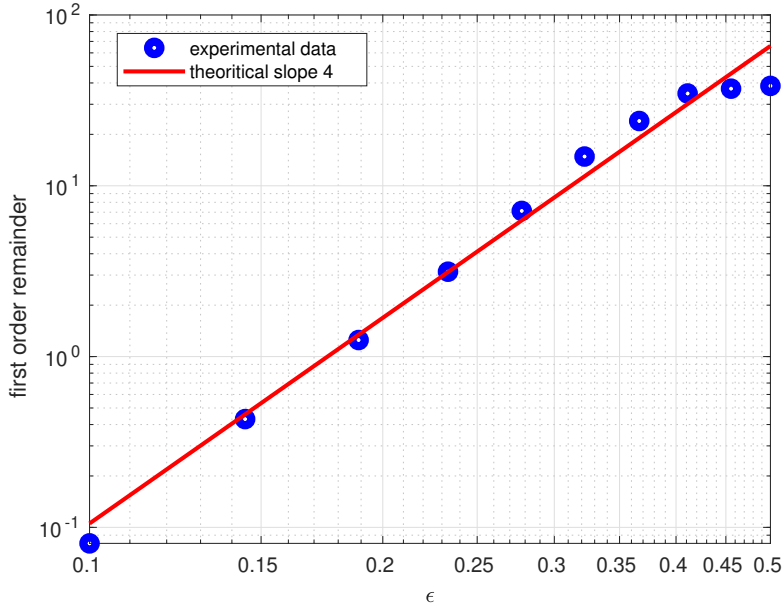
FIGURE 7. Values of \mathfrak{E} as a function of the radius \epsilon of the two spherical particles in a log-scale. The slope of the solid line is 4 .
