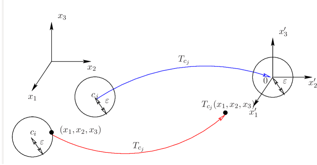
FIGURE 3. Effect of the translation of the coordinates system for several particles.
