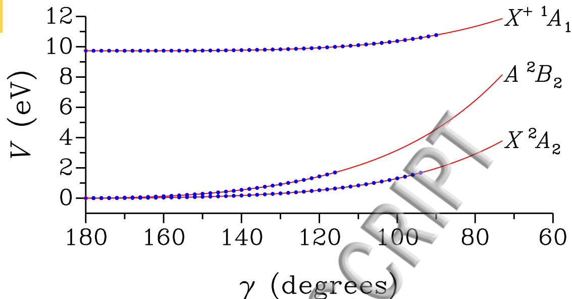
Figure 1. Variations with the bending angle \gamma = \angle\text{CNC} of the potential energy function V in eV for the X^2A_2 and A^2B_2 electronic substates of the CNC radical resulting from the RT coupling and for the X^1A_1 electronic state of the \text{CNC}^+ cation. Ab initio potential values are indicated by dots. Solid lines are the fitted bending potentials calculated with Eq. (1).
