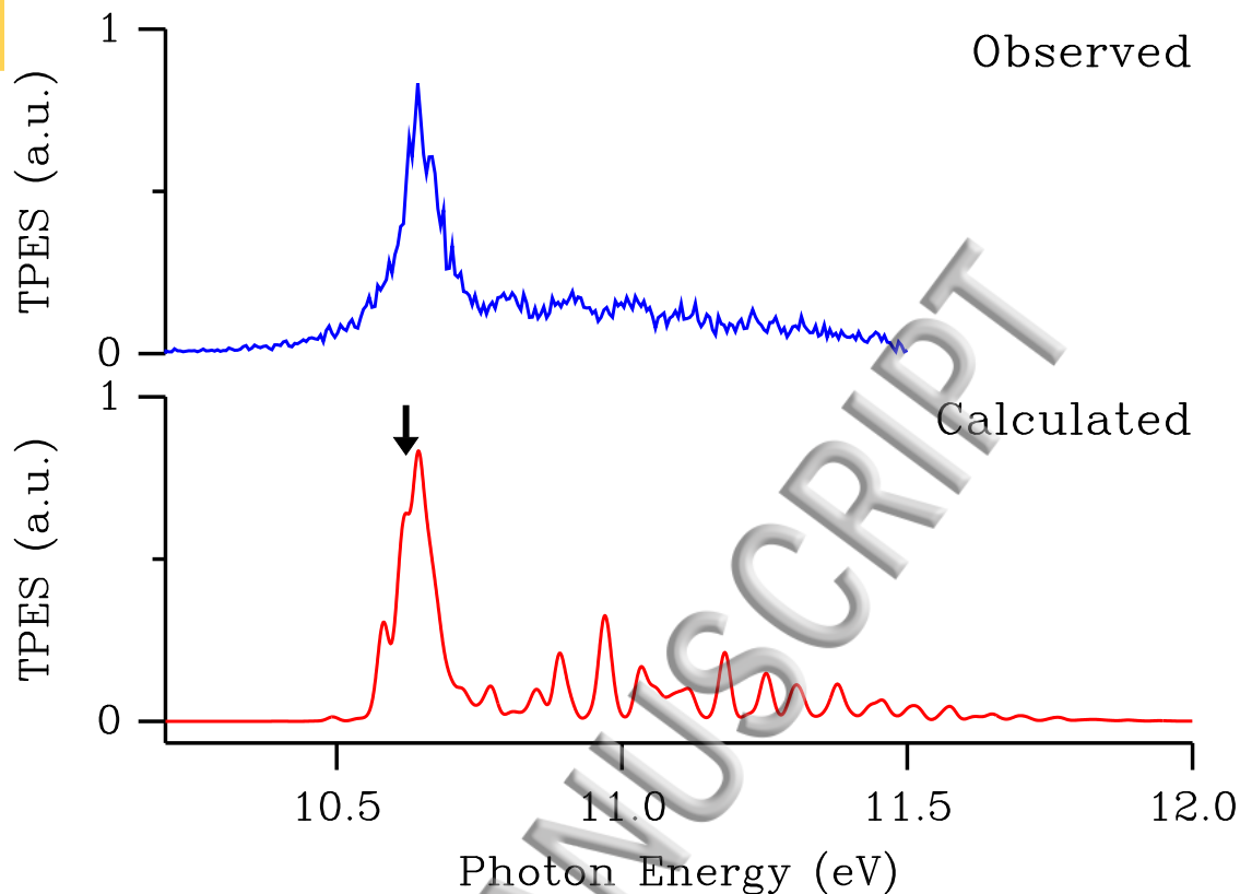
Figure 9. Observed 6 (Calculated) TPES of the X^+ 2\Pi \leftarrow X^3A'' ionizing transition of HCCN in the upper (lower) panel. In the lower panel, the small vertical arrow is the adiabatic ionization potential.
