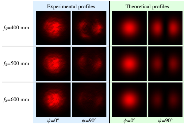
Fig. 3. Linear shearing interferograms of light focused by lenses implemented holographically via a SLM. In each row, from the top down, f_s = 400 mm, 500 mm and 600 mm. The first and third columns contain respectively the experimental and theoretical profiles for \psi = 0 , while the second and fourth columns show the same for \psi = 90^\circ . The plates' separation is \zeta = 12.0 mm.
