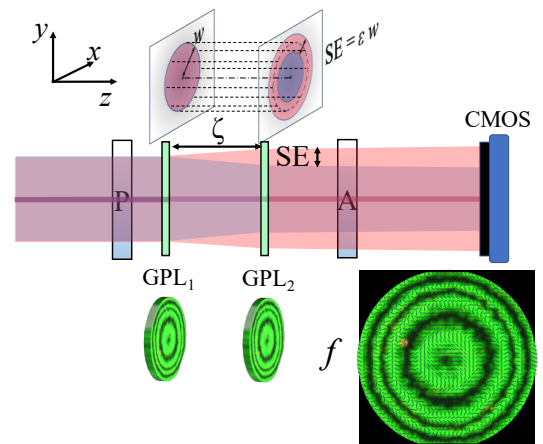
Fig. 6. Sketch of a radial GPSI. This device is identical to the GPSI in Fig. (1), but with the \Lambda -plates replaced by GPLs with focal length f = (130 \pm 1) mm. The bottom-right inset shows the fast-axis distribution of the GPLs we fabricated, superimposed onto the experimental polarization fringe pattern of the GPL.
