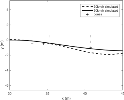
Fig. 3 Avoidance trajectories
