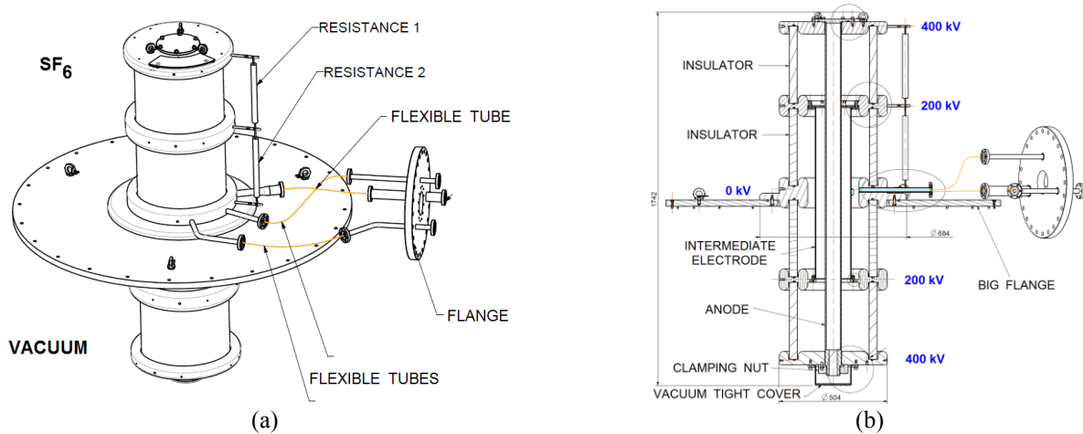
FIGURE 7. (a) 3D view of the bushing. (b) Cut-through view of the bushing.
