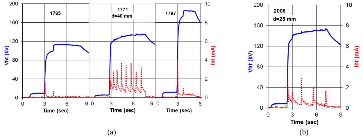
FIGURE 6. (a) Voltage V_{ht} (blue solid line) and power supply current I_{ht} (red dotted line) vs. time for three pulses: 1765 no N_2 , no dark current; 1771 no N_2 , dark current; 1787 with 0.1 Pa N_2 . The distance between the electrodes was 40 mm. (b) Voltage and power supply current for pulse 2008, electrodes separated by 25 mm, no N_2 .
