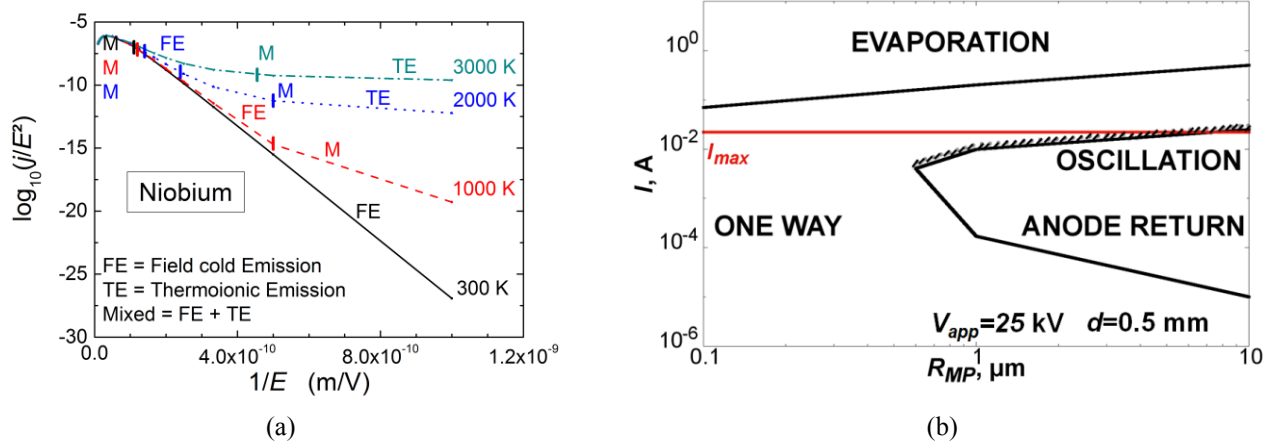
FIGURE 2. (a) Family of Fowler-Nordheim-like characteristics of the electron emitted current from a micro-tip for several tip temperatures indicating the coexistence of Field Emission (FE) and Thermionic Emission (TE). (b) Different regimes of MP dynamics versus the MP radius ( R_{MP} ). The figure corresponds to a constant voltage V = 25 kV and gap distance d = 0.5 mm.
