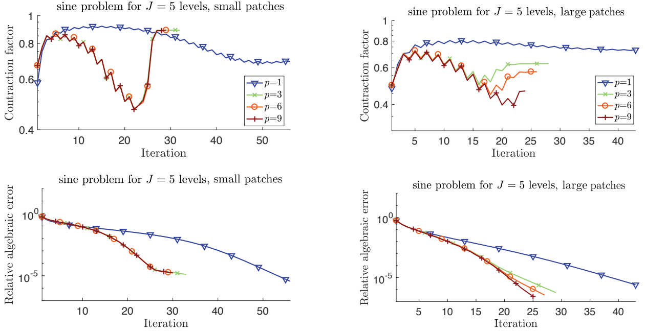
Figure 3: Sine problem (6.1), w_1 = J(d + 1) , w_2 = 1 : results of the solver (4.6) for p' = p in (2.10a), “small” (left) and “large” (right) patches, and stopping criterion (6.4); top: error contraction factors \|\nabla(u_J - u_J^{i+1})\|/\|\nabla(u_J - u_J^i)\| ; bottom: relative algebraic error \|\nabla(u_J - u_J^i)\|/\|\nabla u_J\| .
